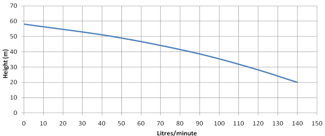
Pump Performance
